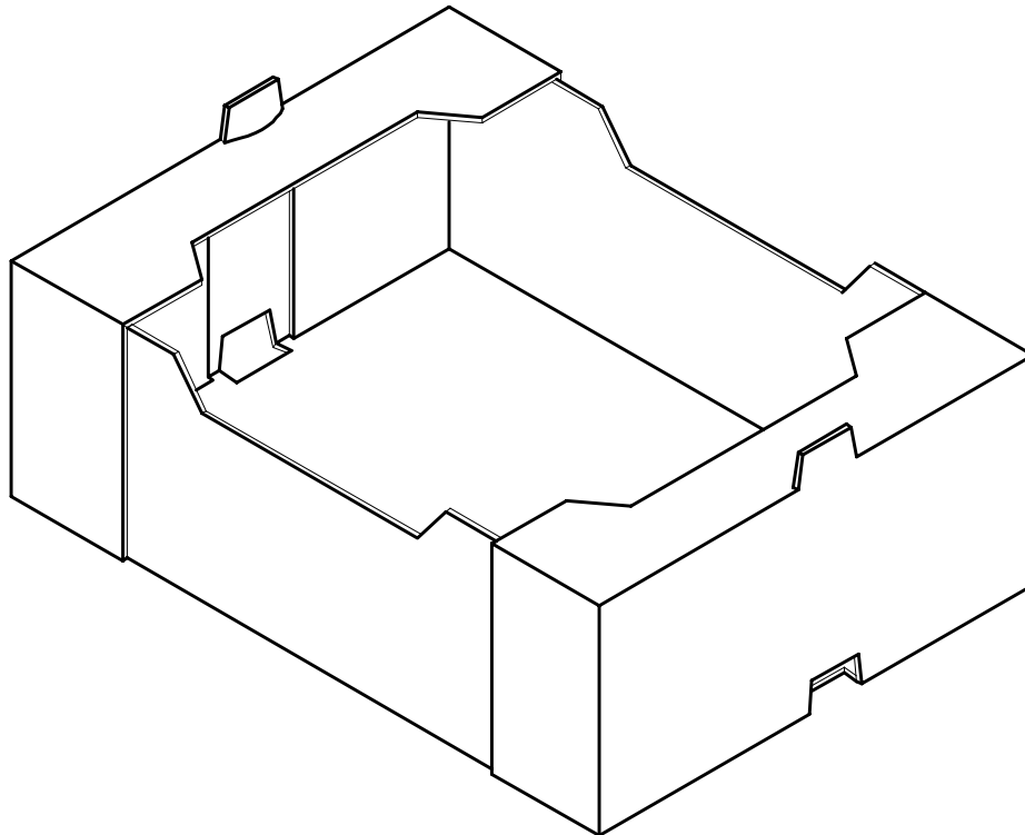
ILLUSTRATION #1B TRAY CORNER FLANGE SEAL BLUEBERRY BOX
