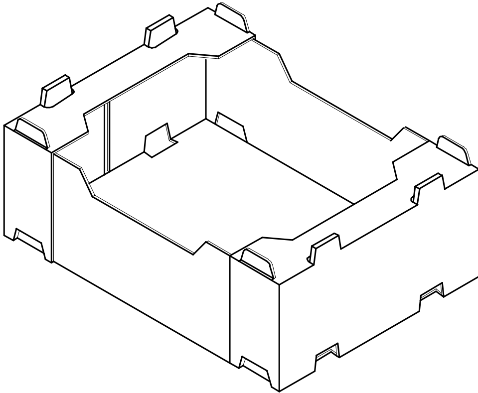
ILLUSTRATION #6 CORNER FLANGE SEAL PEACH DISPLAY TRAY
