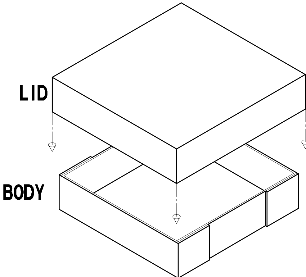
ILLUSTRATION #11E TWO PIECE TELESCOPE POULTRY EXPORT TRAY WITH OUTSIDE MINOR FLAPS ON BODY
