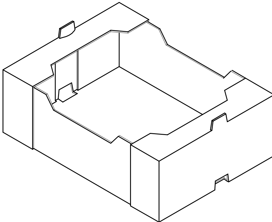
ILLUSTRATION #1C TRAY CORNER FLANGE SEAL BLUEBERRY BOX
