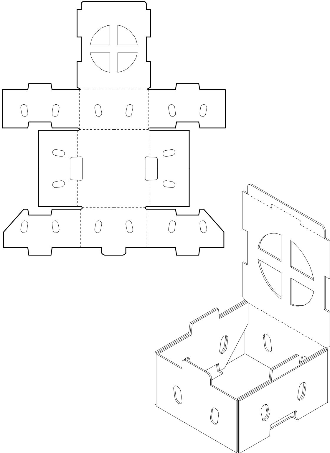
ILLUSTRATION #6 CITRUS DISPLAY STYLE W/ OVERLAPPING MINOR FLAPS
