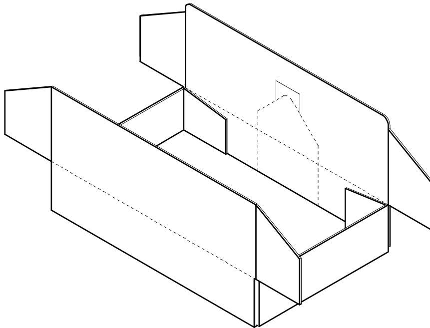
ILLUSTRATION #7A TRAY STYLE W/ TOP TUCK IN FLAPS
