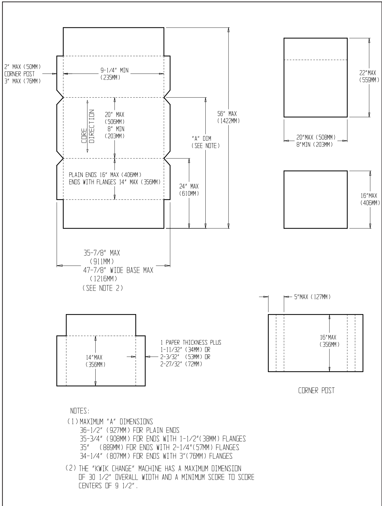
Figure 1-1: Bliss Box Specifications
